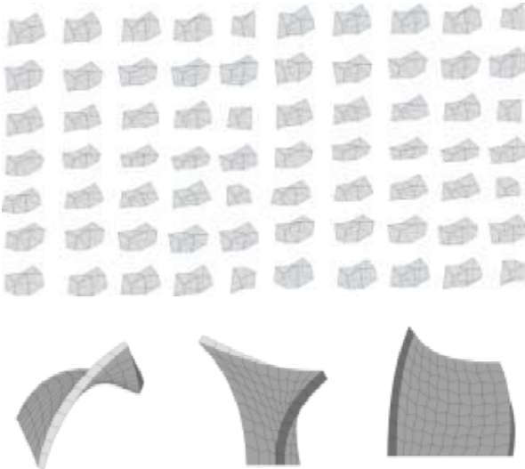
Fig. 12. Prototype A: geometric configuration and individual bricks.
