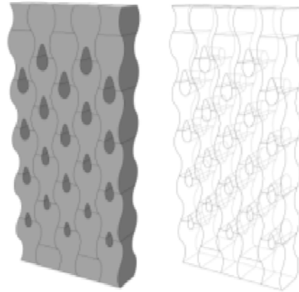
Fig. 14. Prototype B: geometric configuration
