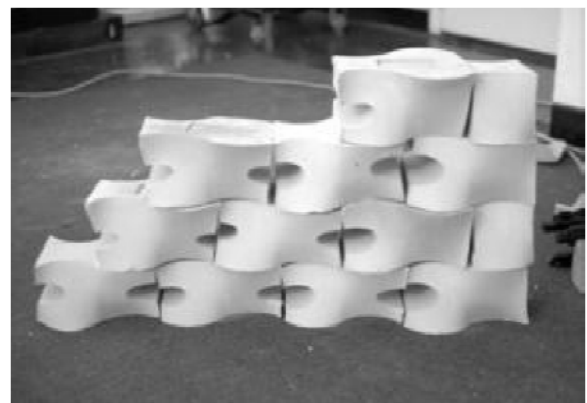
Fig. 15. Prototype B: unfired ceramic elements and partial assembly simulation
